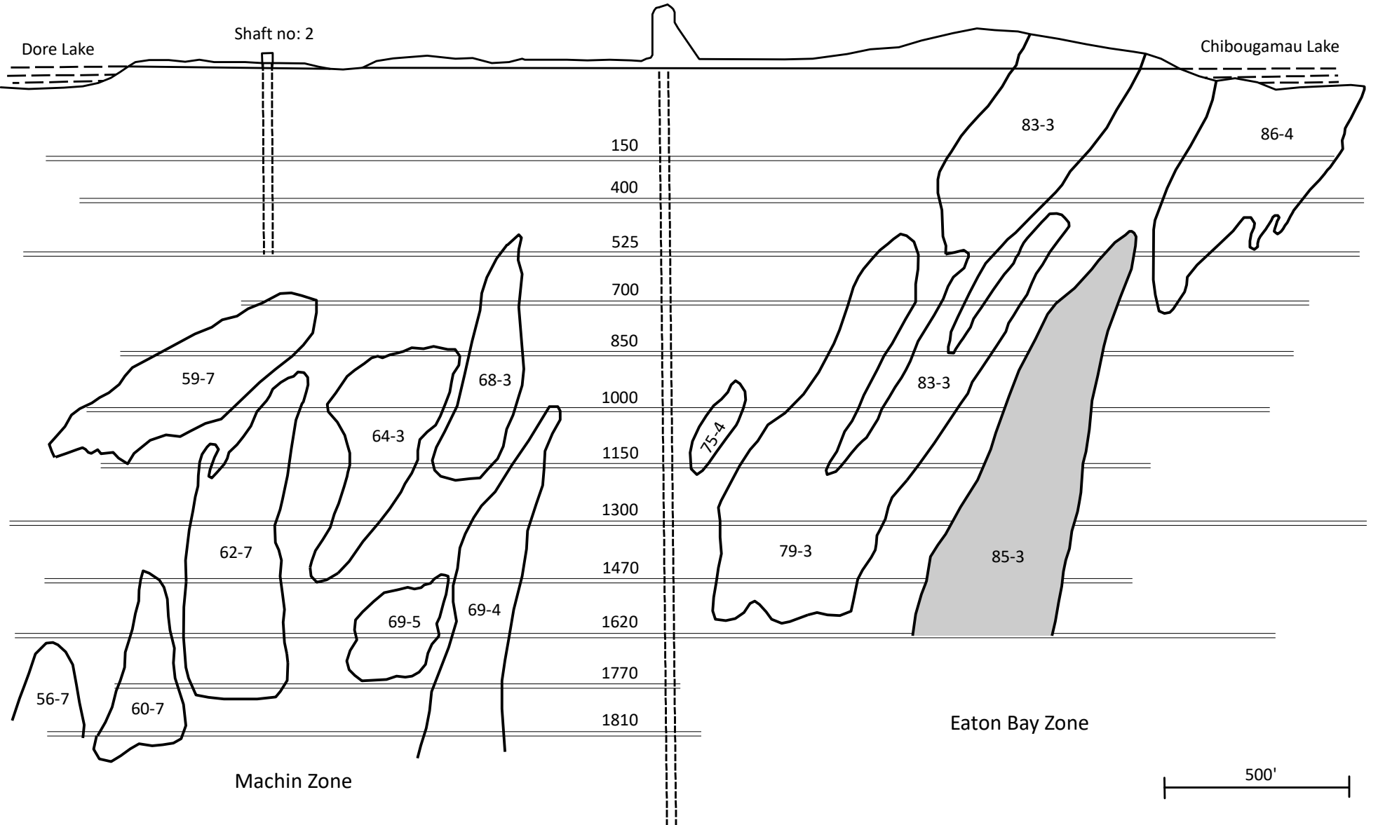
Longitudinal Section - Upper Portion Copper Rand Mine by André Tremblay, Department of Applied Sciences University of Quebec, Chicoutimi - 1980
